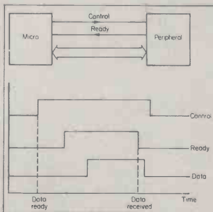
Figure 8. Output handshake.
